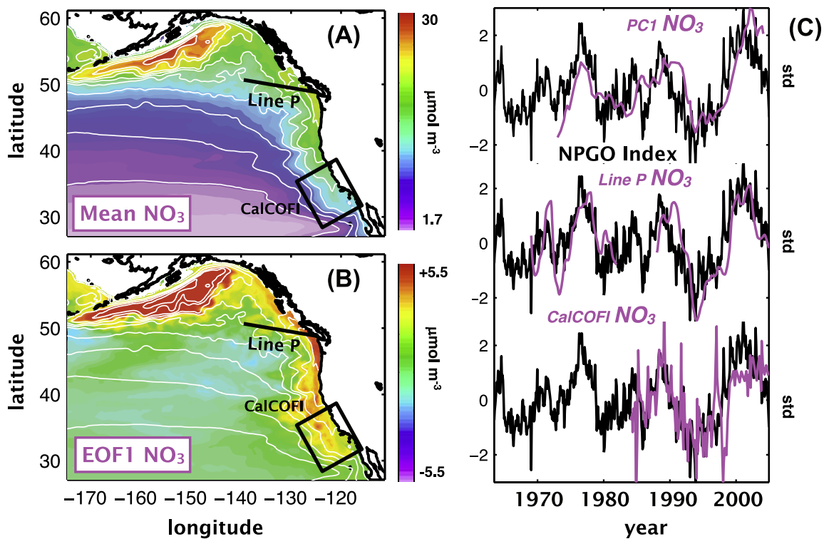
Figure 3. Temporal and spatial variability of subsurface nitrate (NO 3 ). (a) Mean subsurface (150 m) NO 3 from ROMS ocean model over the period 1975–2004. (b) First mode of variability for model subsurface (150 m) NO 3 anomaly inferred from EOF1. White contours mark the mean NO 3 distributions in Figures 3a and 3b. (c) Timeseries of NPGO index (black) compared to PC1 of NO 3 ( R = 0.65 , 99%), observed mix layer NO 3 at Line-P [Peña and Varela, 2007] ( R = 0.68 , 99%), and observed NO 3 from CalCOFI program ( R = 0.51 , 95%). All timeseries are normalized by their standard deviations, units are in standard deviations (std).
