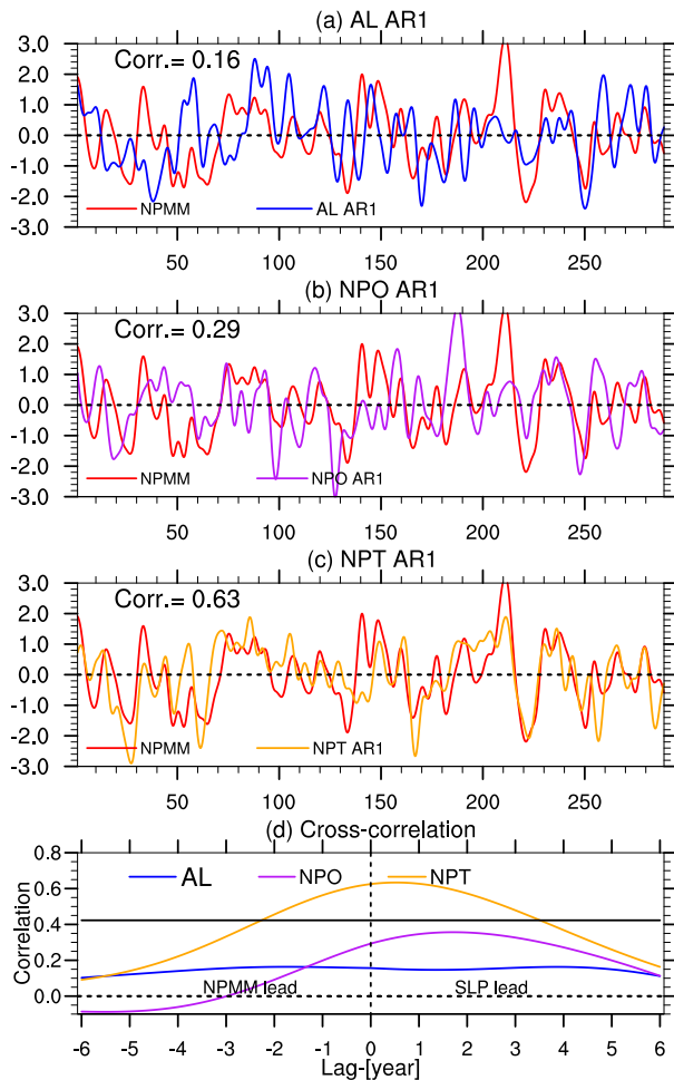
FIG. 10. The 10-yr low-pass filtered reconstructed NPMM time series based on the AR-1 model, as reconstructed by (a) AL variability, (b) NPO variability, and (c) NPT variability. Red lines denote the SST EC of decadal NPMM variability. Correlation between the low-pass filtered reconstructed NPMM time series and the SST EC is marked in each panel. (d) Cross-correlation between the SST EC of decadal NPMM variability and 10-yr low-pass filtered reconstructed NPMM time series forced by AL (blue), NPO (purple), and NPT (yellow) variability based on the AR-1 model. Horizontal solid line denotes the correlation at 95% confidence interval based on the two-tailed Student's t test.
