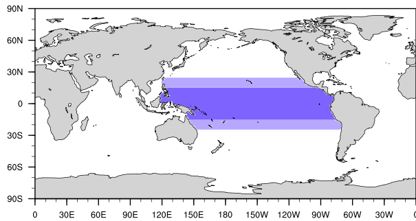
FIG. 1. Schematic of the Clim- \tau experiment. Dark blue shading indicates the region where daily climatological wind stress is prescribed (15°S–15°N). Light blue shading denotes the buffer zones to the north (15°–25°N) and south (25°–15°S). Otherwise, the ocean and atmosphere are fully coupled and free to evolve.
