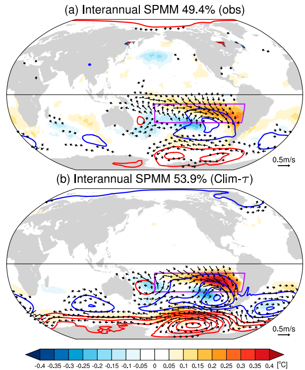
FIG. 11. As in Fig. 4, but for interannual SPMM.
